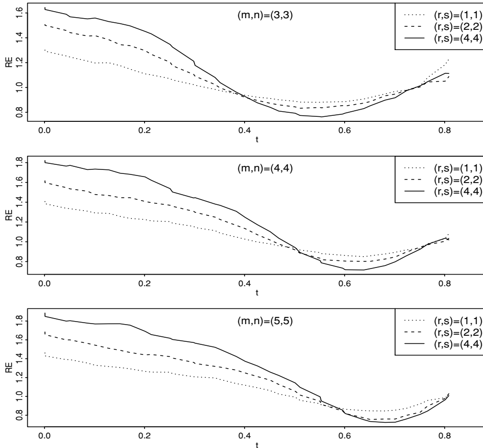
FIGURE 1. Estimated REs for F(x) = x, 0 < x < 1 , and \sigma = 0.85 .
