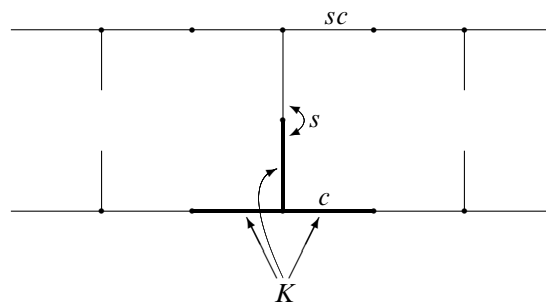
Figure 1: Cocycles x and x \cdot s
