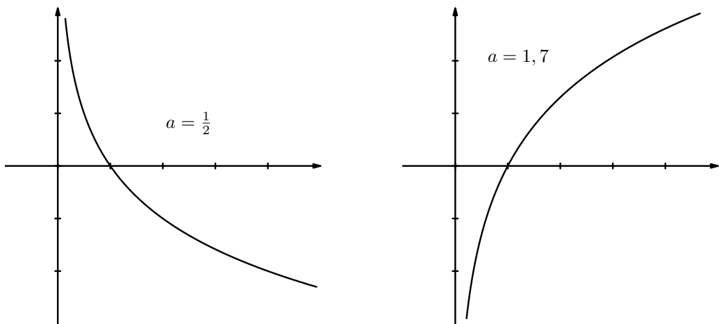
Figure 3.5: Logarytm f(x) = \log_a x .
