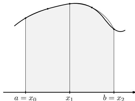
Figure 14.2: Metoda Simpsona, n = 2 .
