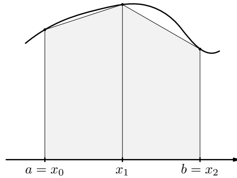
Figure 14.1: Metoda trapezów, n = 2 .
