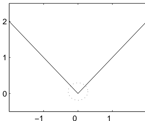
Figure 8.2: The graph of f(x) = |x| and the non-differentiable “angle”.
