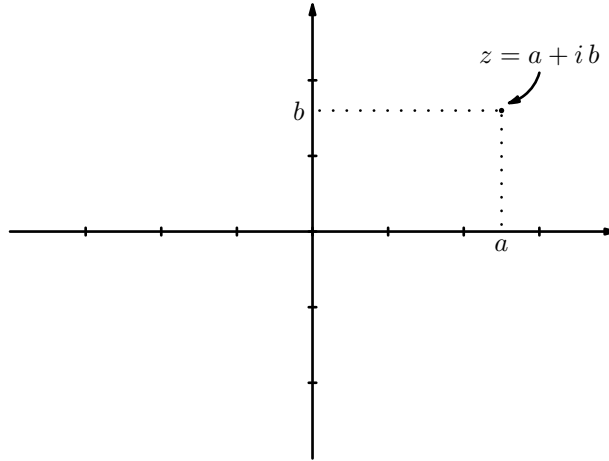
Figure 2.3: Complex plane.
