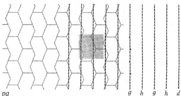
pg
