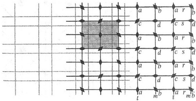
pmm
