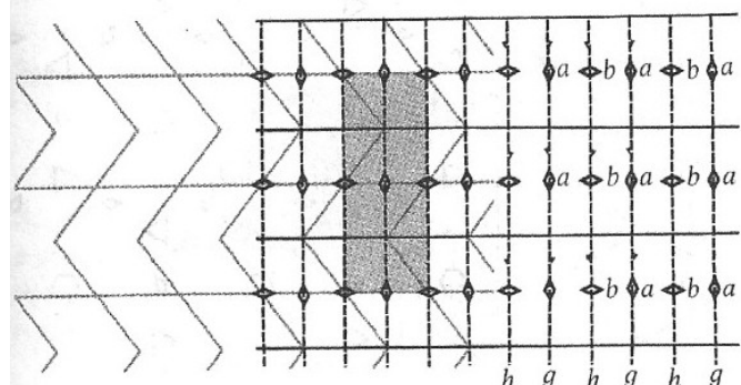
pmg
