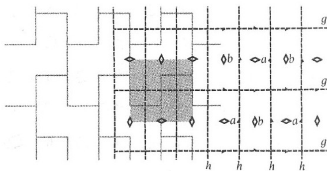
pgg
