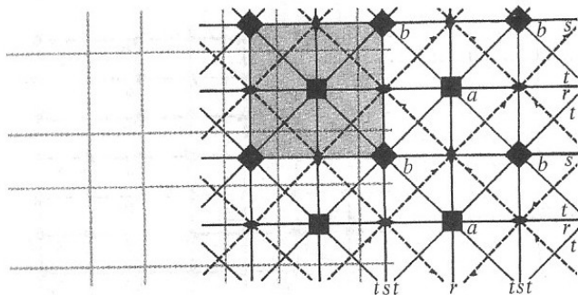
p4m
