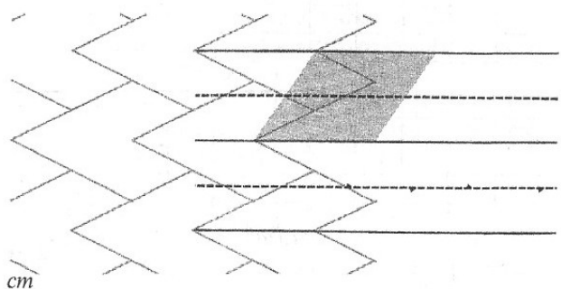
cm
