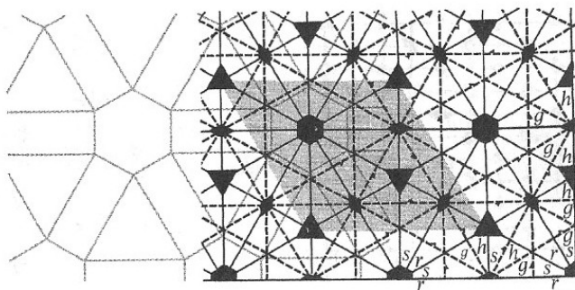
p6m
