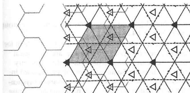
p31m
